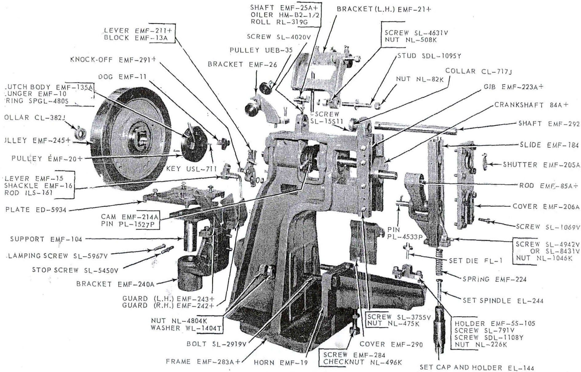
Figure 8 - Exploded View of Machine
